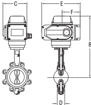
Lug Valve with Electric Actuator
