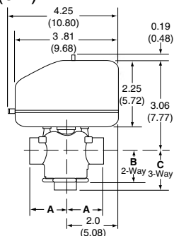
Spring Return
