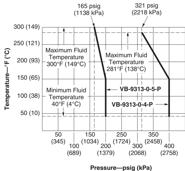
Figure 2. Temperature and Pressure Ratings for VB-9313 Series Valve Bodies.
