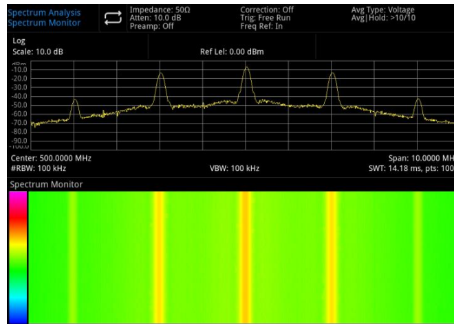
Figure 5-6 Spectrum Monitoring
