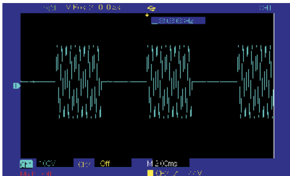
Figure 3 - 4 OSK waveform with oscilloscope
