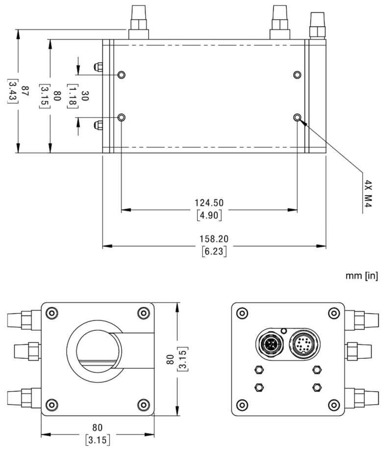
Figure 8-18: Enclosure Dimensions
