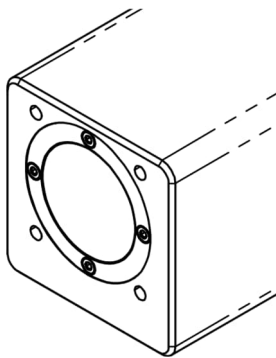
Figure 8-24: Protective Window
