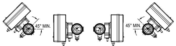
Figure 4: Mounting rotation
