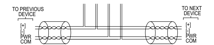
Figure 1: Common local power supply
