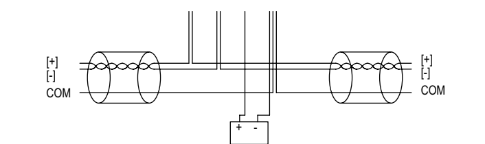
Figure 2: Local power supply
