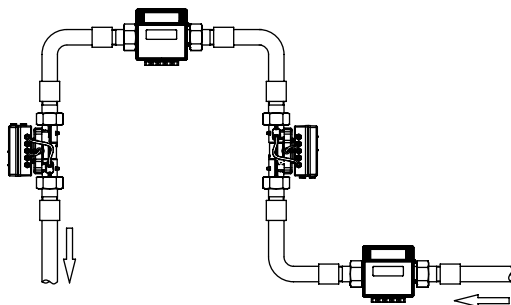
Figure 3: Installation positions
