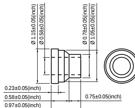
½" DN15-UNION-PP SDR 11 IR FUSION
