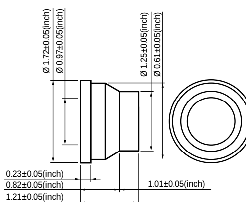
1" DN25-UNION-PP SDR 11 IR FUSION
