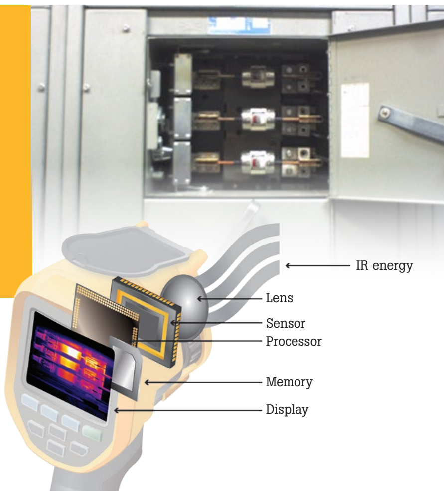
Figure 1. Anatomy of an infrared camera
