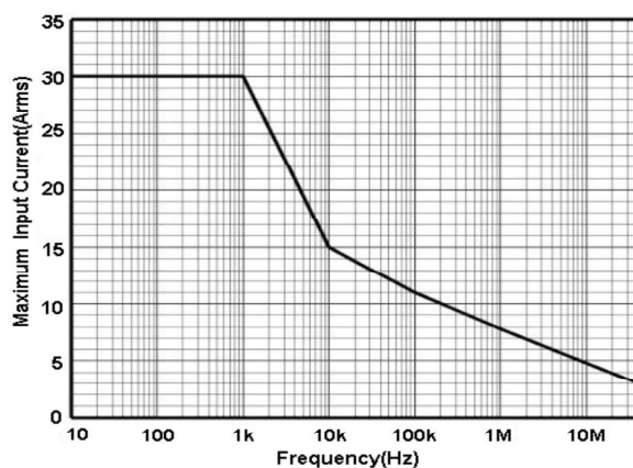
T3CP30-50 Continuous Maximum Current Input
