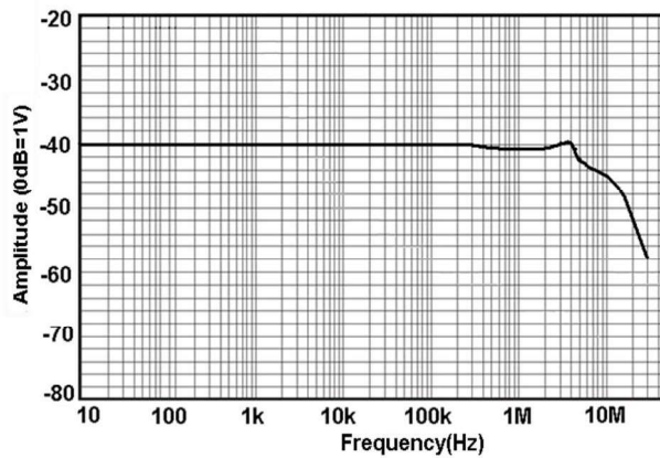
T3CP500-5 Frequency Response
