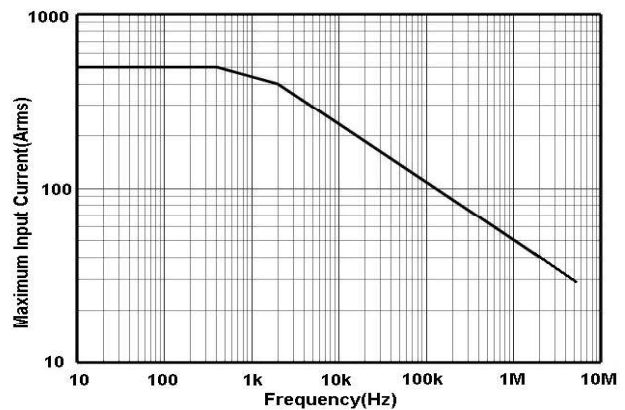
T3CP500-5 Continuous Maximum Current Input
