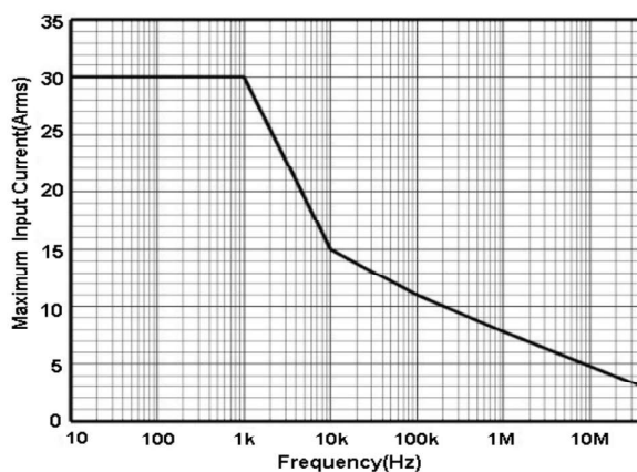
T3CP30-50 Continuous Maximum Current Input
