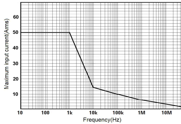
T3CP50-50 Continuous Maximum Current Input
