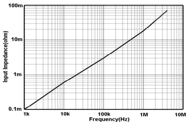
T3CP500-5 Insertion Impedance
