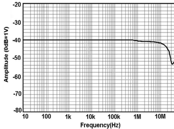
T3CP150-12 Frequency Response
