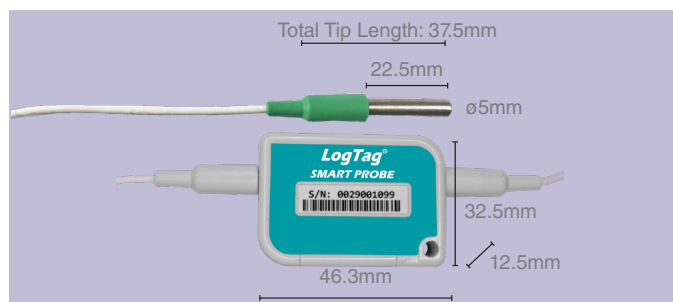
CP10S - Smart Probe
