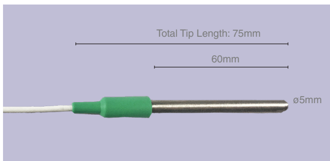
ST10M - Medium Round Tip Probe
