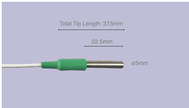
ST10S - Short Round Tip Probe
