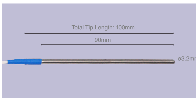
ST100L - Long Round Tip Probe
