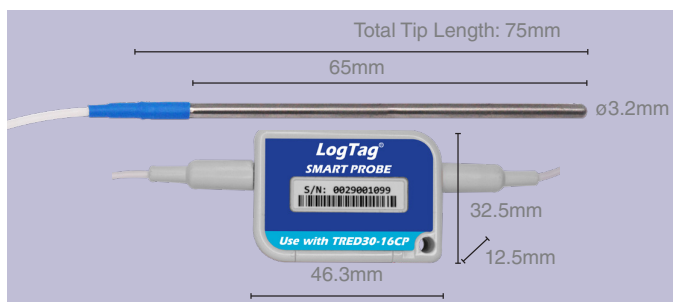
CP110K - Smart Probe
