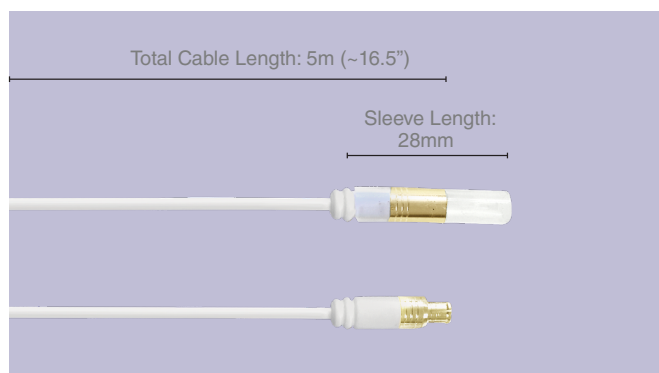
STX-50 - External Probe Extension cable
