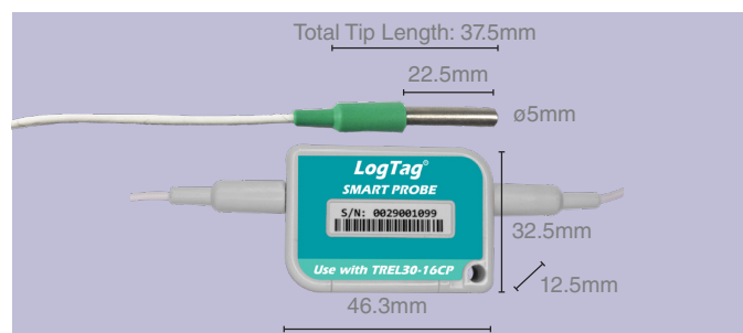
CP11S - Smart Probe
