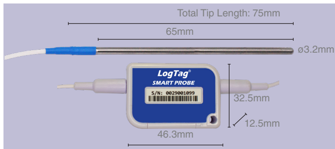
CP100K - Smart Probe
