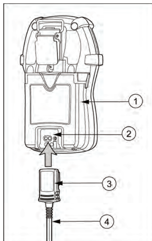
Figure 16. Connecting the Charger Adapter
