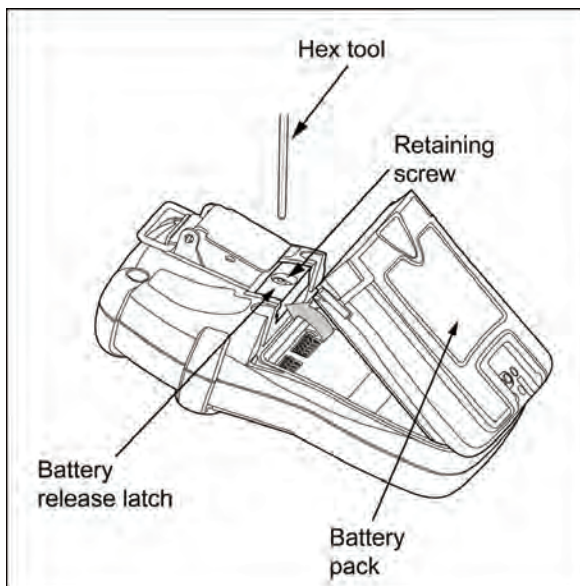
Figure 18. Removing the Battery Pack
