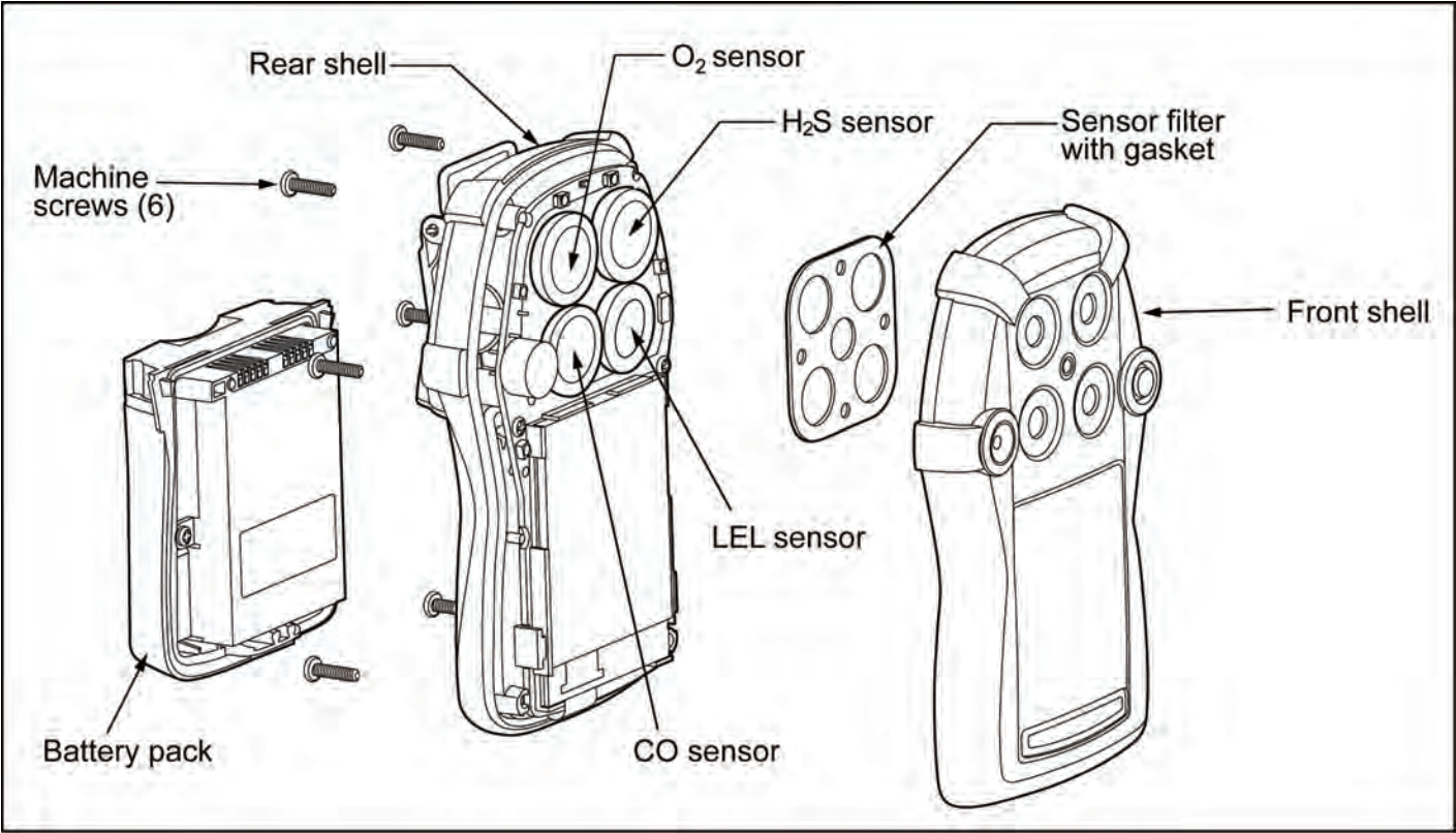
Figure 23. Replacing a Sensor or Sensor Filter
