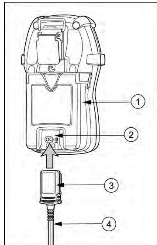
Figure 2. Connecting the IR Link
