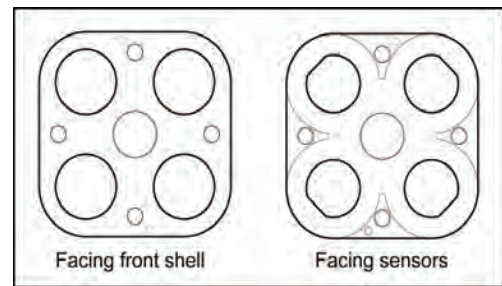
Figure 25. Inserting the Sensor Filter Correctly
