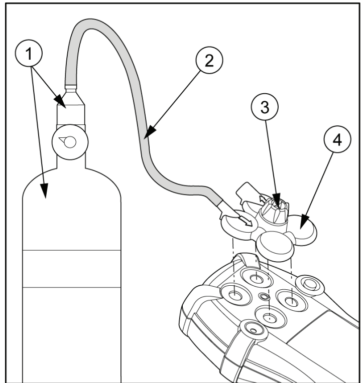
Figure 8. Bump Test Installation
