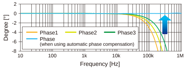
Example of the automatic phase compensation for the AC/DC current sensor
