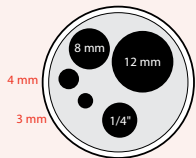
Multi-hole M08
