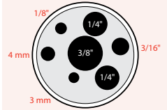
Multi-hole M06
