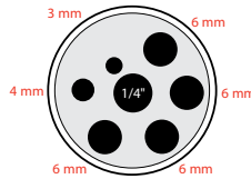
Multi-hole M02
