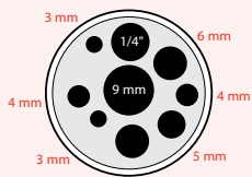
Multi-hole M04
