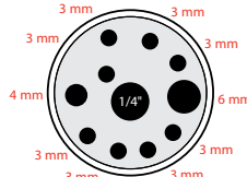
Multi-hole M03
