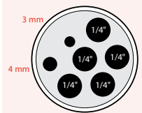
Multi-hole M05
