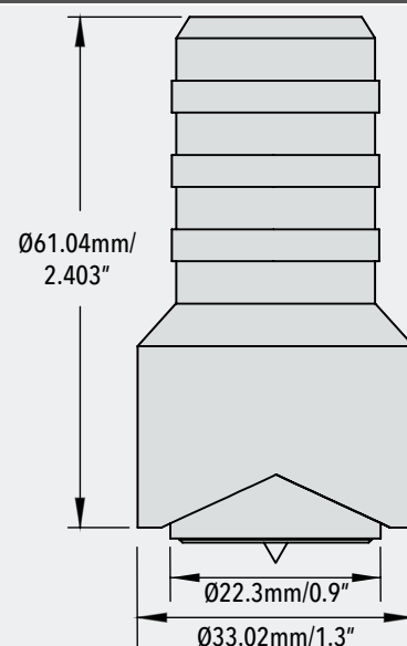
PosiTector SPGOS
