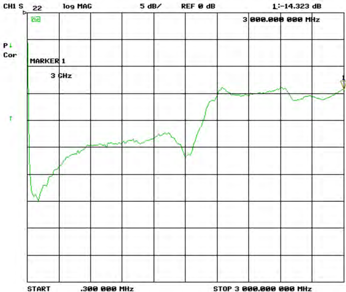
Image 15 - Wideband amplifier output return loss, IS22I 300 kHz to 3 GHz lin.
