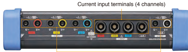
Voltage input terminals (4 channels; channels 1/2/3 and channel 4 are isolated from each other)
