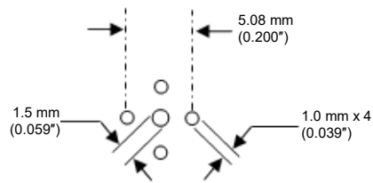
PC Board hole size and pattern
