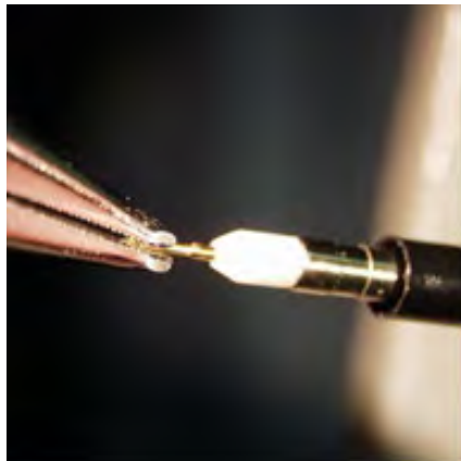
To remove tips, grip the outermost portion and pull straight out.
