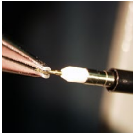
To remove tip, grip the spring-loaded portion beyond the outer sleeve and pull straight out.
