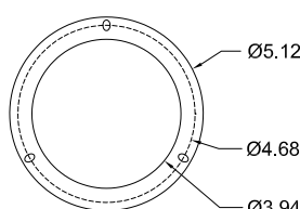
4" MOUNTING FLANGE
