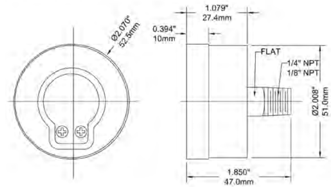
2" Back Connection
