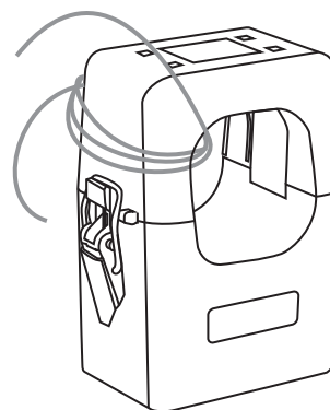
Figure 1: PDA6405 Current Transformer Shown with Four Turns
