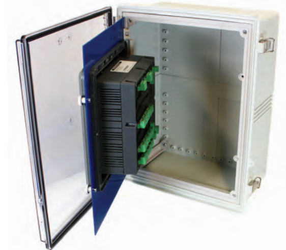
PDA3939 plastic enclosure open with clear cover and interior door for mounting ConsoliDator+
