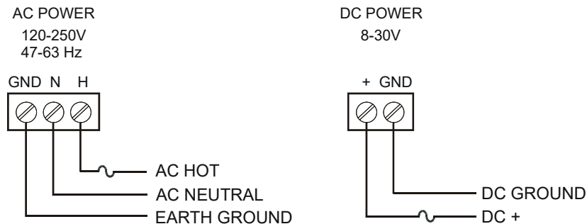
Figure 3. Power Connections
