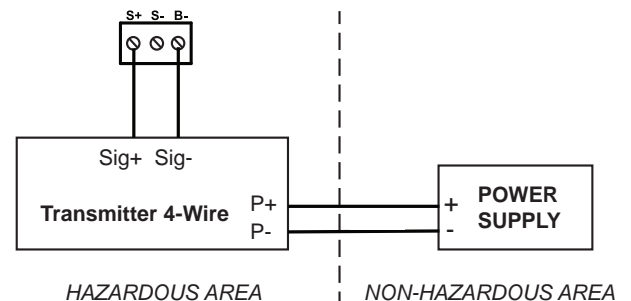
Figure 6: Control Loop Connections with Backlight (4-Wire)
