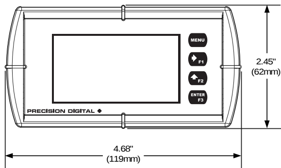
▲ Meter Dimensions - Front View
