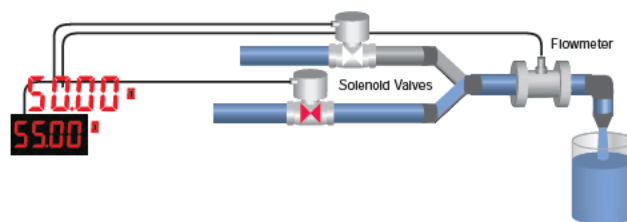
Multi-Stage Batch Control
