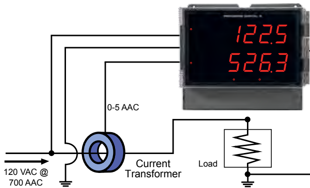
Voltage/Current Input Application Example
