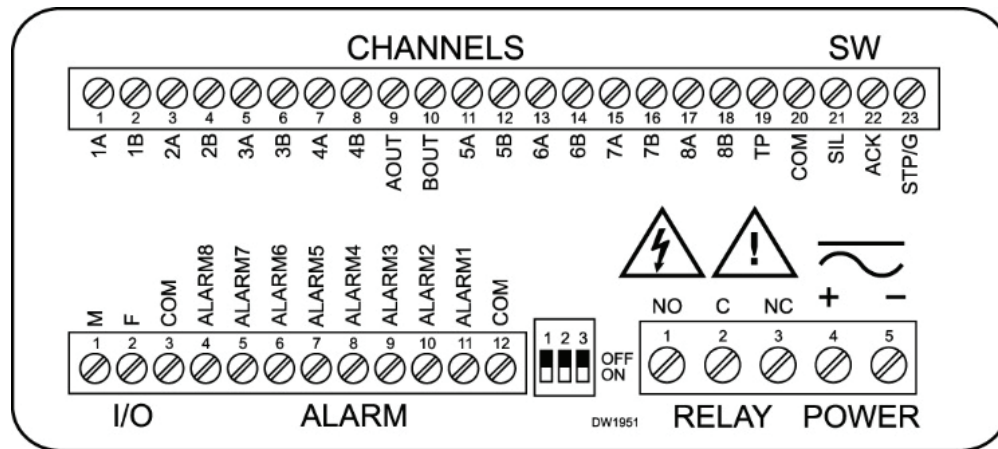
Figure 2. Connector Labeling for PD138
