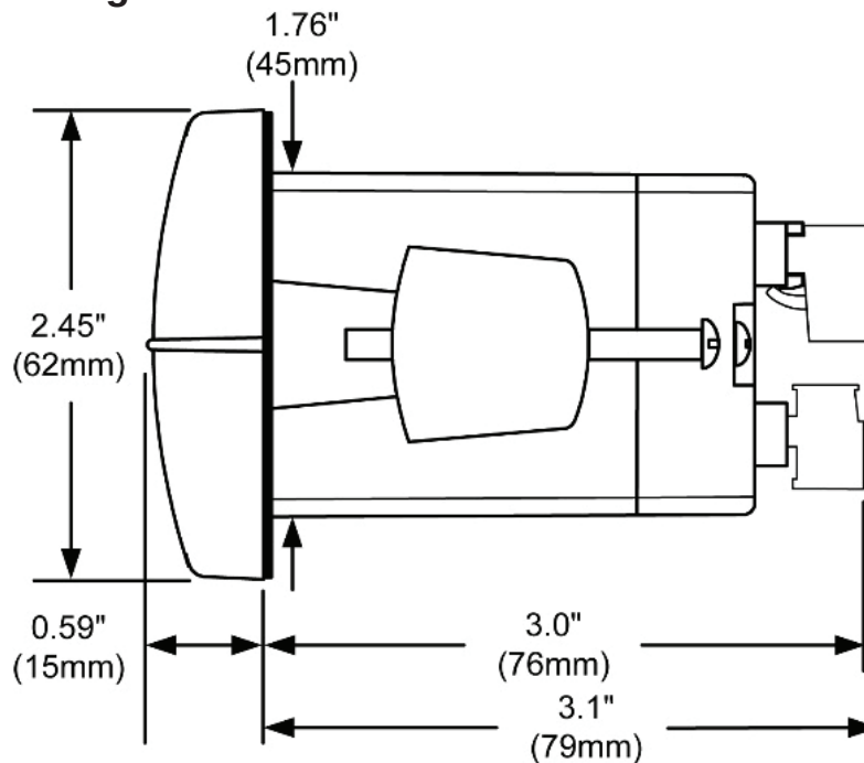
Figure 3. Case Dimensions – Side View
