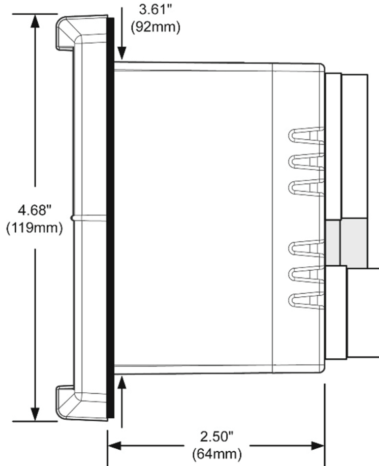
Figure 3. Case Dimensions – Side View
