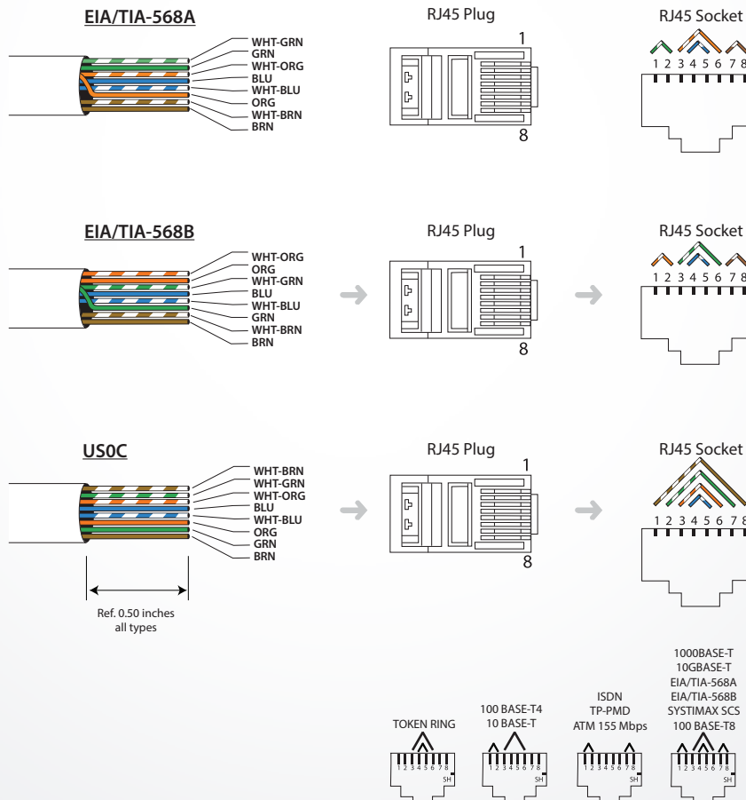
RJ45 Cable Connection
