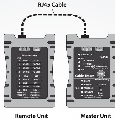
RJ45 Cable Connection
