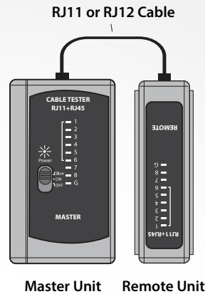
RJ11/RJ12 Cable Connection
