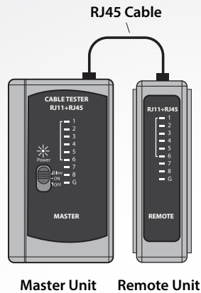
RJ45 Cable Connection
