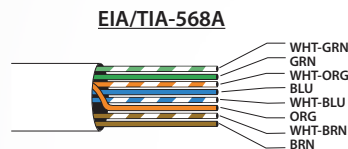
RJ45 Cable Connection
