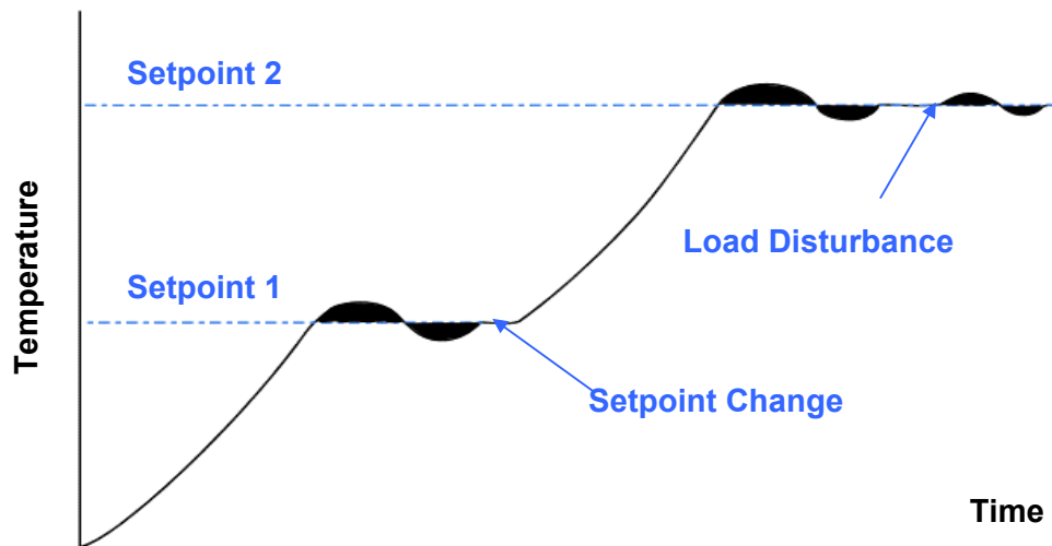
Figure 45. Self-Tune Operation
