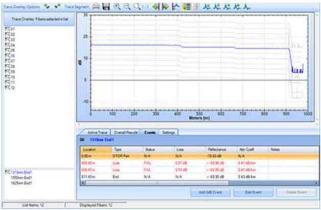
Batch Processing and stack traces in LinkWare PC
