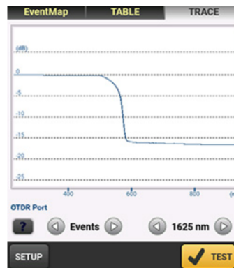
Splitter as seen on an OTDR trace
