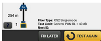
Link with an APC connector shown as a loss event
