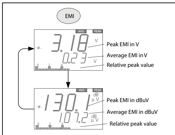
Figure 12. EMI Measurement screen
