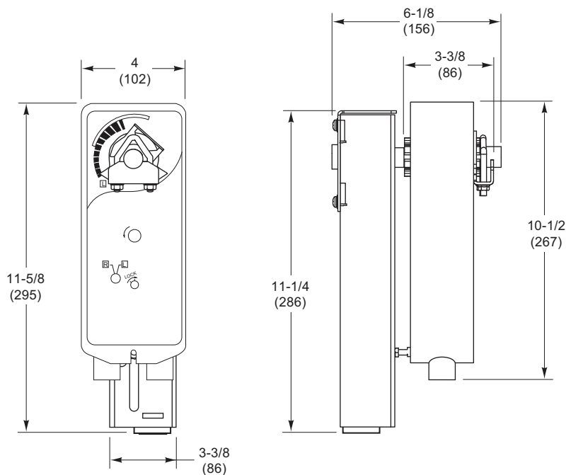
Figure-29 Mx41-715x or Mx41-707x Linked Actuator Assembly With AV-602 Linkage.
