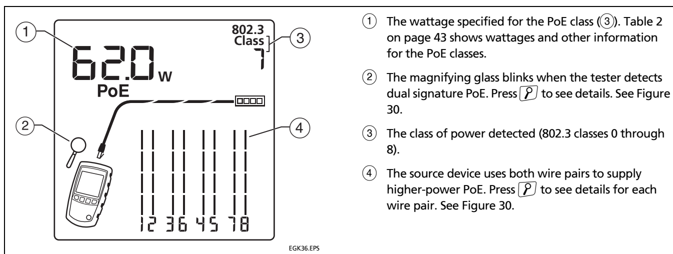
Figure 29. PoE from a Dual-Signature PoE Source (MicroScanner PoE)
