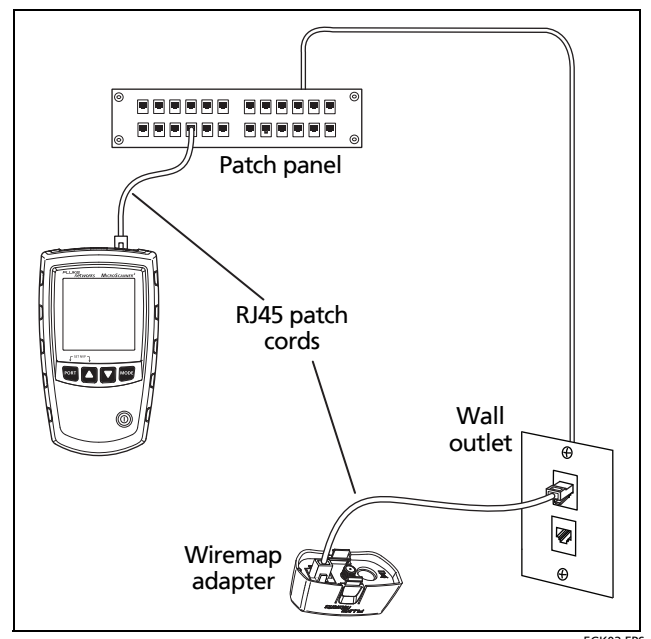
Figure 7. Connecting to Twisted Pair Network Cabling
