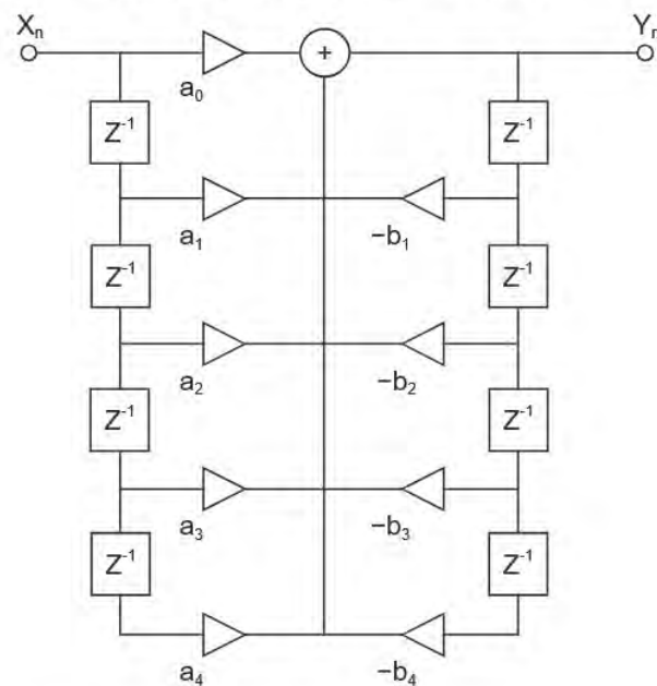
IIR filter configuration (4th-order IIR filter)
