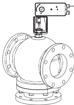
Vx-8303/Vx-9313 with Mx61-720x Direct-Mounted Actuator
