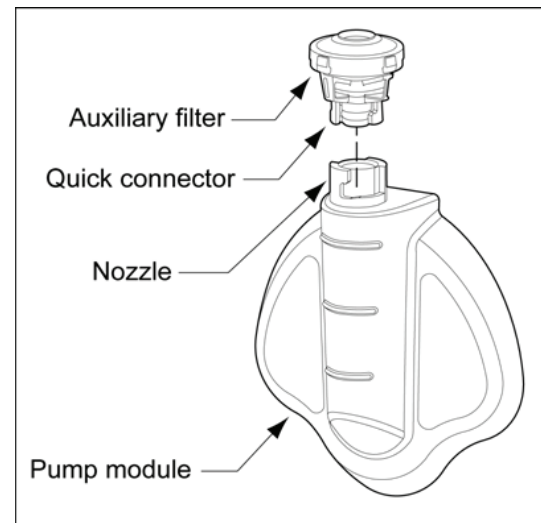
Figure 9. Attaching the Auxiliary Filter
