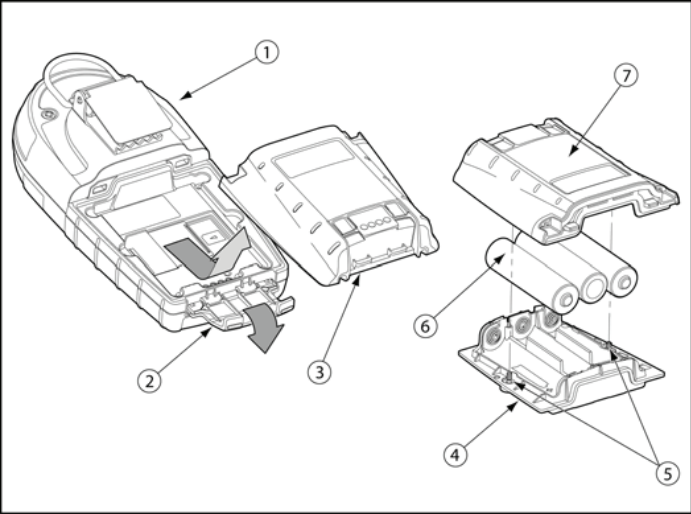
Figure 13. Replacing the Alkaline Batteries
