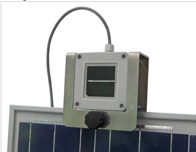
Mounting of Irradiation Reference Sensor on a PV-Modul
