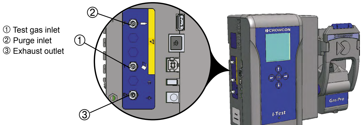
Figure 2: Inlet/exhaust connections
