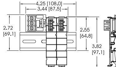
IQRL-2002 (AC Power Only)
