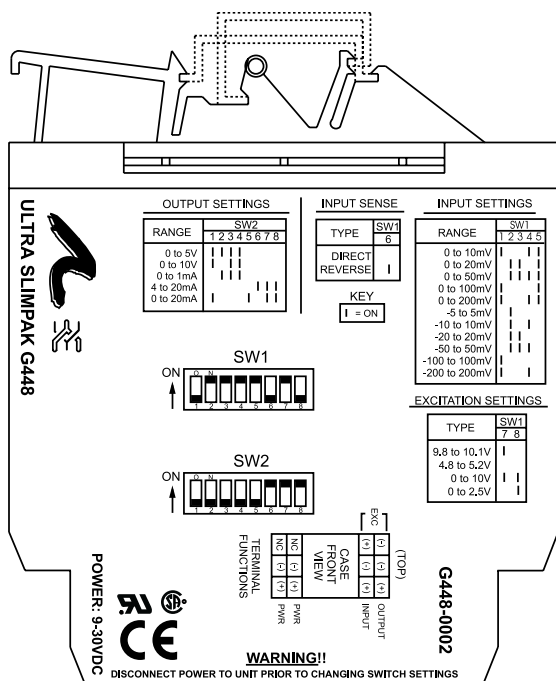
Figure 1: G448 Factory Cal: 0 to 30mV (0 -50mV Switch Settings) 10V Excitation, Direct Operation, 4-20mA Output
