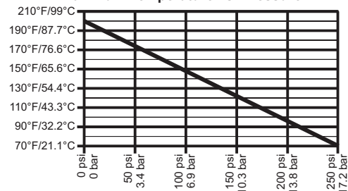
Maximum Temperature vs. Pressure
