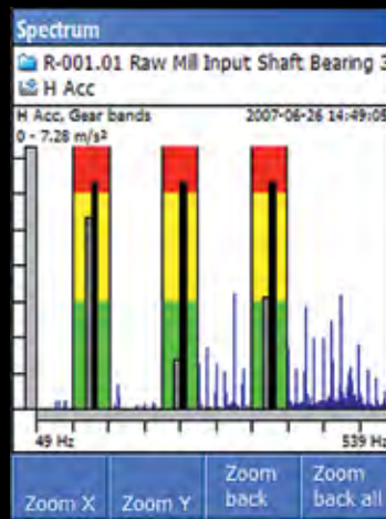
SPM HD spectrum with bands for trending
