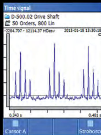
Time signal from an SPM HD measurement
