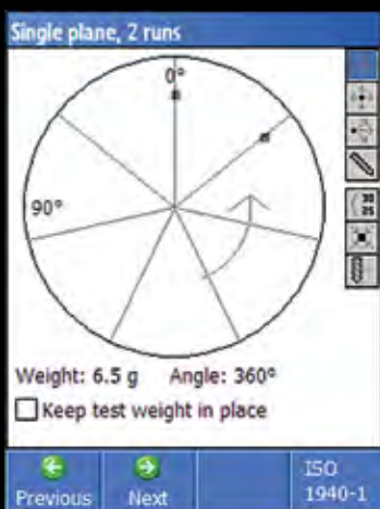
Dynamic balancing in single plane according to ISO 1940-1
