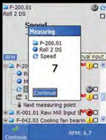
Speed measurement and High Definition Order Tracking
