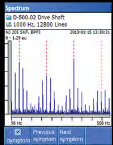
Vibration spectrum from an EVAM measurement
