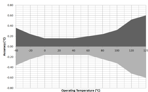
'Type A' Thermistor Probe - sold separately Part number: EL-PROBEA-3.0M-TP+
