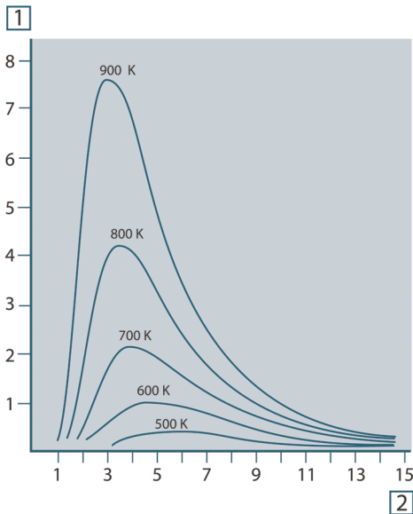
Figure 29.4 Blackbody spectral radiant emittance according to Planck's law, plotted for various absolute temperatures. 1: Spectral radiant emittance (W/cm 2 × 10 3 ( \mu\text{m} )); 2: Wavelength ( \mu\text{m} )
