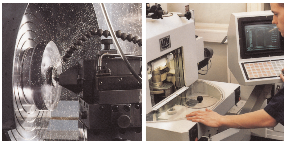
Figure 25.4 LEFT: Diamond turning machine; RIGHT: Lens polishing
