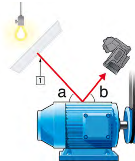
Figure 12.2 1 = Reflection source
