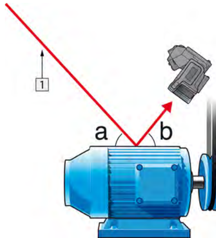
Figure 12.1 1 = Reflection source
